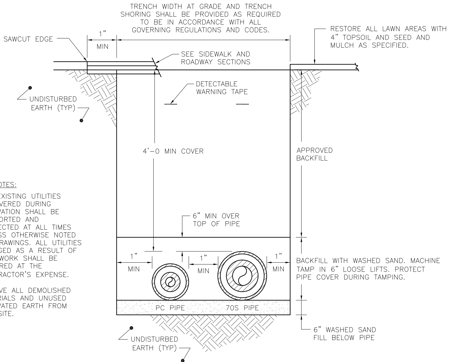
DETAIL STM-17 - STEAM & CONDENSATE DIRECT BURIED SYSTEM UTILITY TRENCH SECTION
