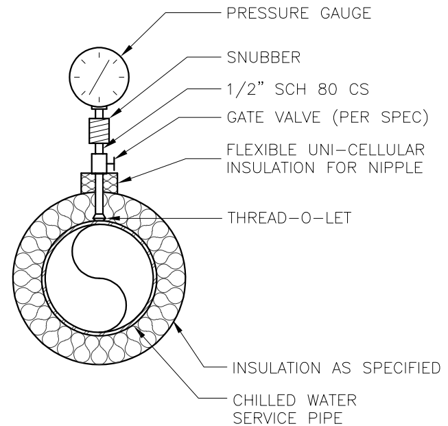
CHILLED WATER
