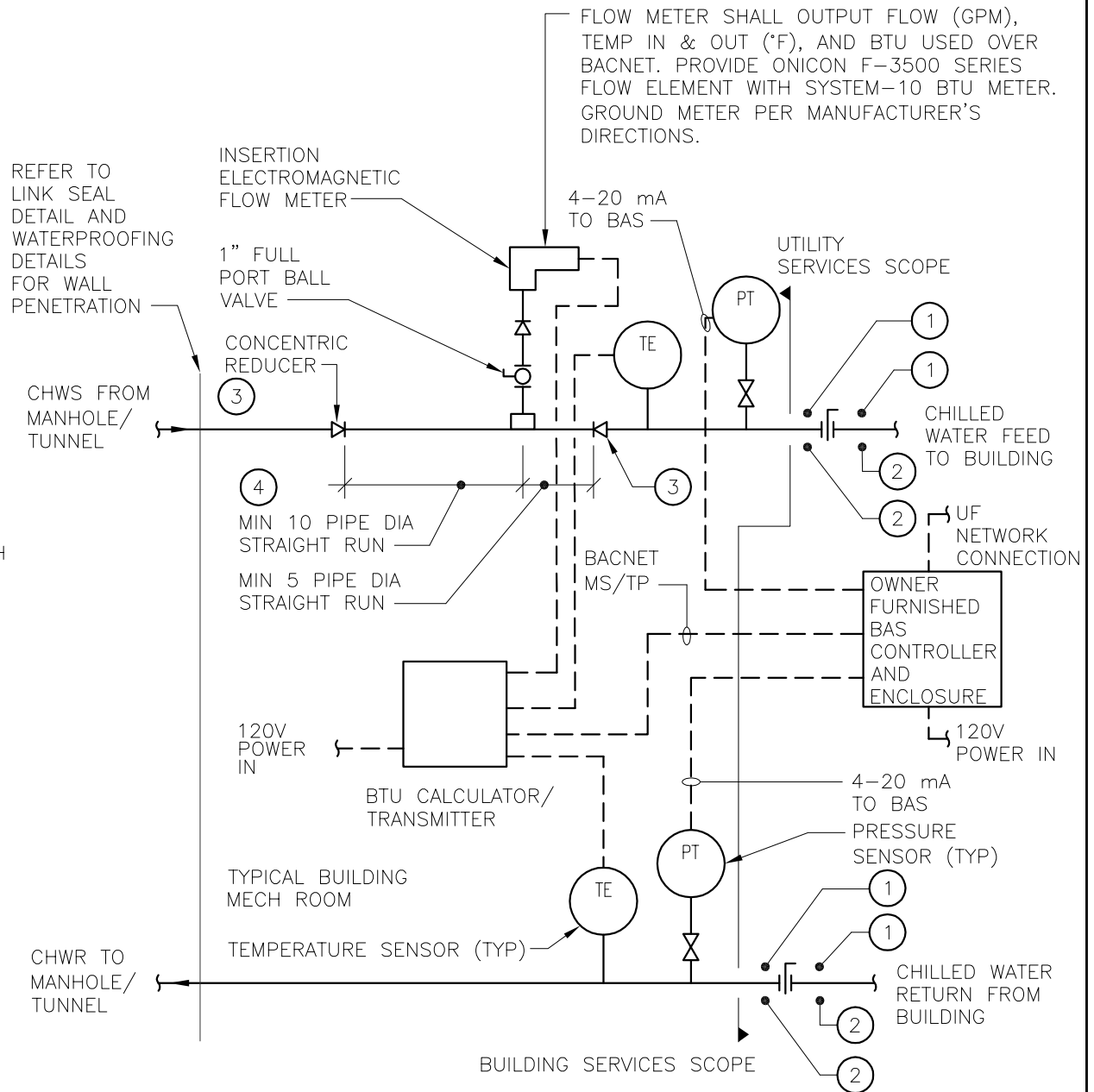
DETAIL CHW-1 - BUILDING CHILLED WATER REQUIREMENTS INCLUDING FLOW METERS
