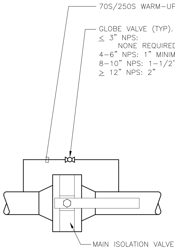
HORIZONTAL PIPE
