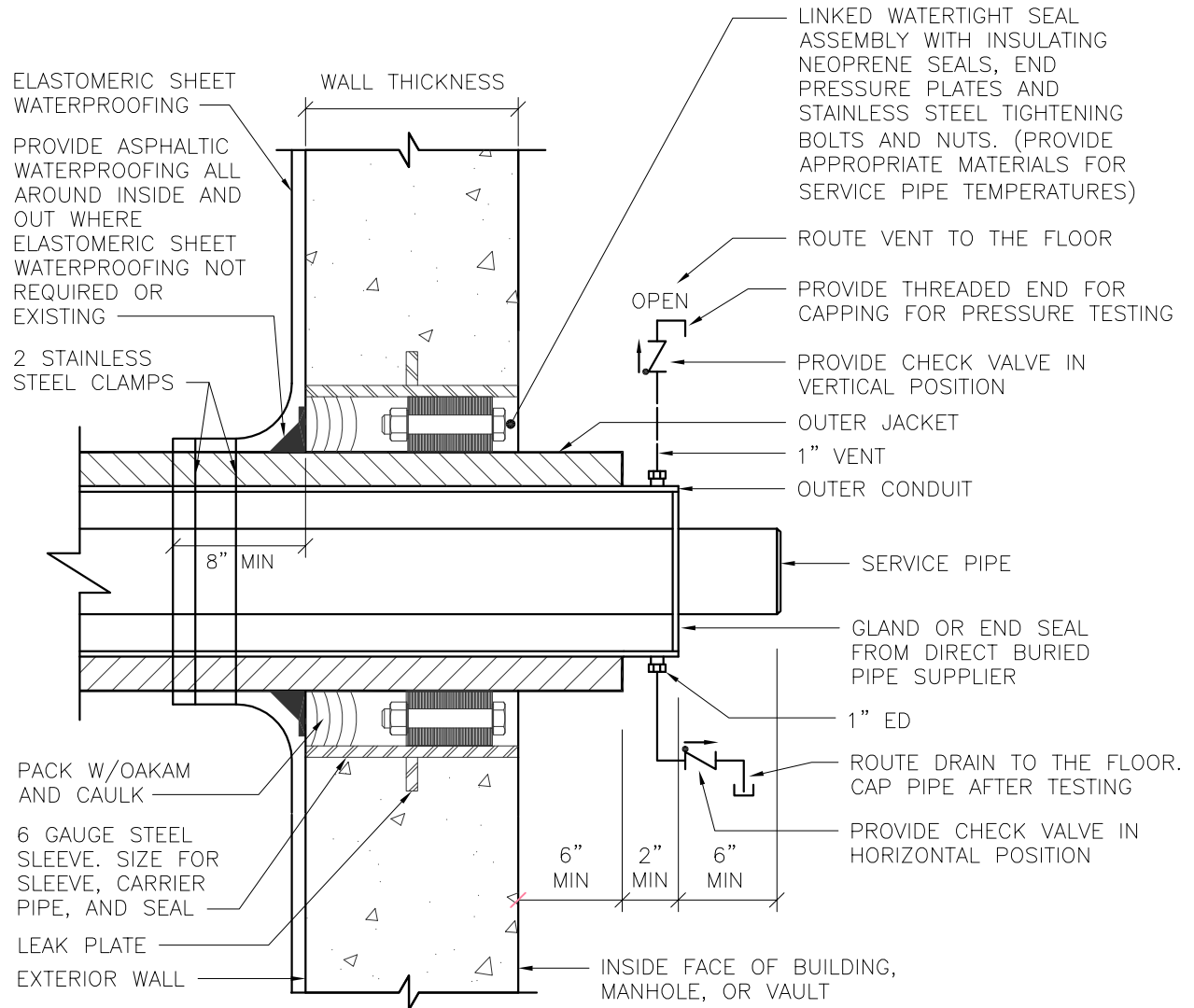
DETAIL MH-8 - WALL PENETRATION
