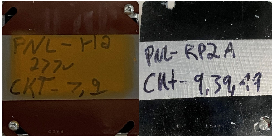
Examples of junction box labeling. 277 / 480 Volt Emergency Power on the left and 120 / 208 Volt on the right.
