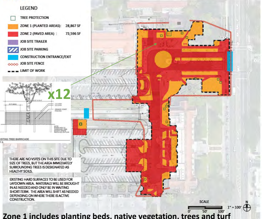
Site plan
