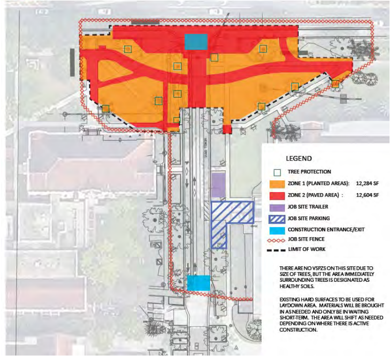
Site plan
